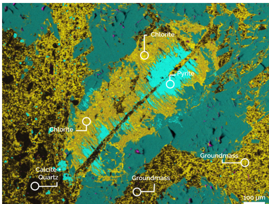
Figure 4.1. Backscatter electron map of metasedimentary anhydrite and mudstone from ~2358 m depth. Relatively aluminum rich regions are represented by magenta, relatively sulfur rich regions are represented by cyan, and relatively magnesium rich regions are represented by yellow. Anhydrite is the dark cyan mineral that is unlabeled on the sample. Relatively large authigenic chlorite surrounds skeletal pyrite.
